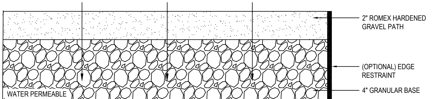
SECTION VIEW
